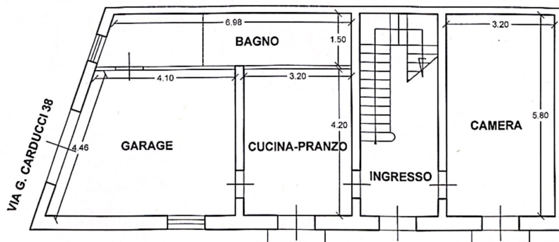
PIANTA PIANO TERRA H= 4.35 ml
